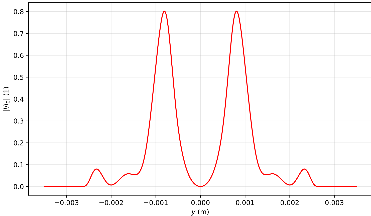
Intensity profile I(x = 0, y, z = 3.981)/I_0 , P_{in}=5.0P_{cr} , artificial time
